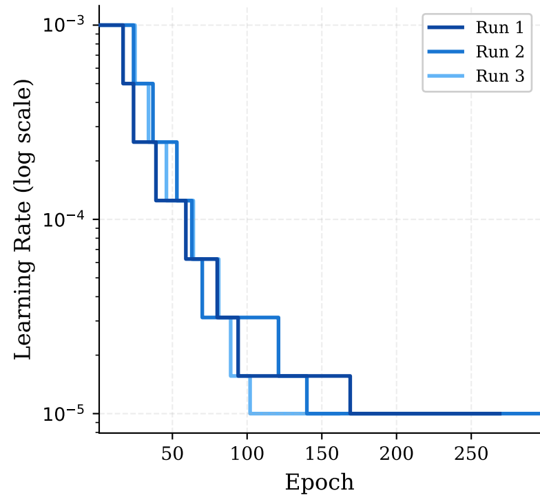
LSTM
