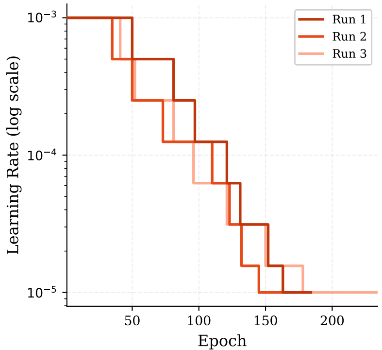
Transformer
