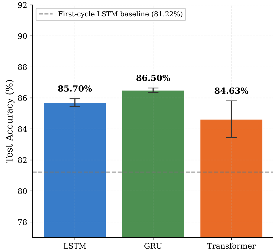
Test Accuracy
