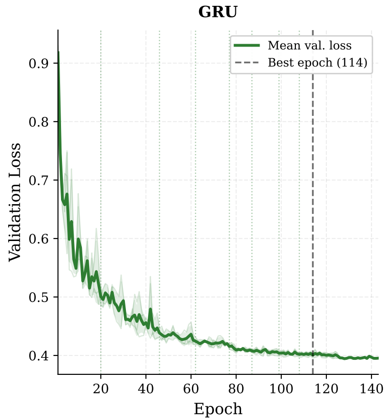
Figure 1 — Validation Loss Convergence Curves
