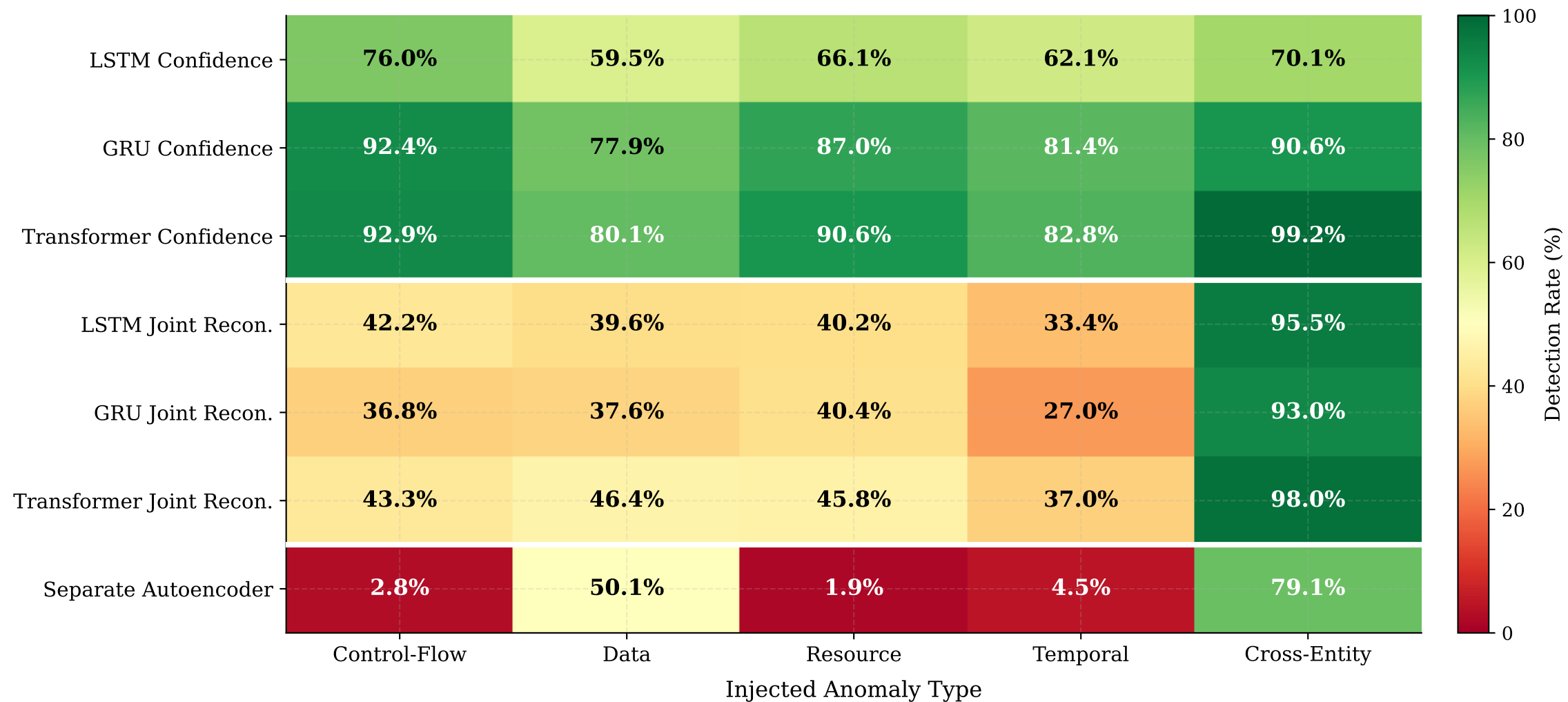
Figure 6 — Per-Type Anomaly Detection Coverage Heatmap
