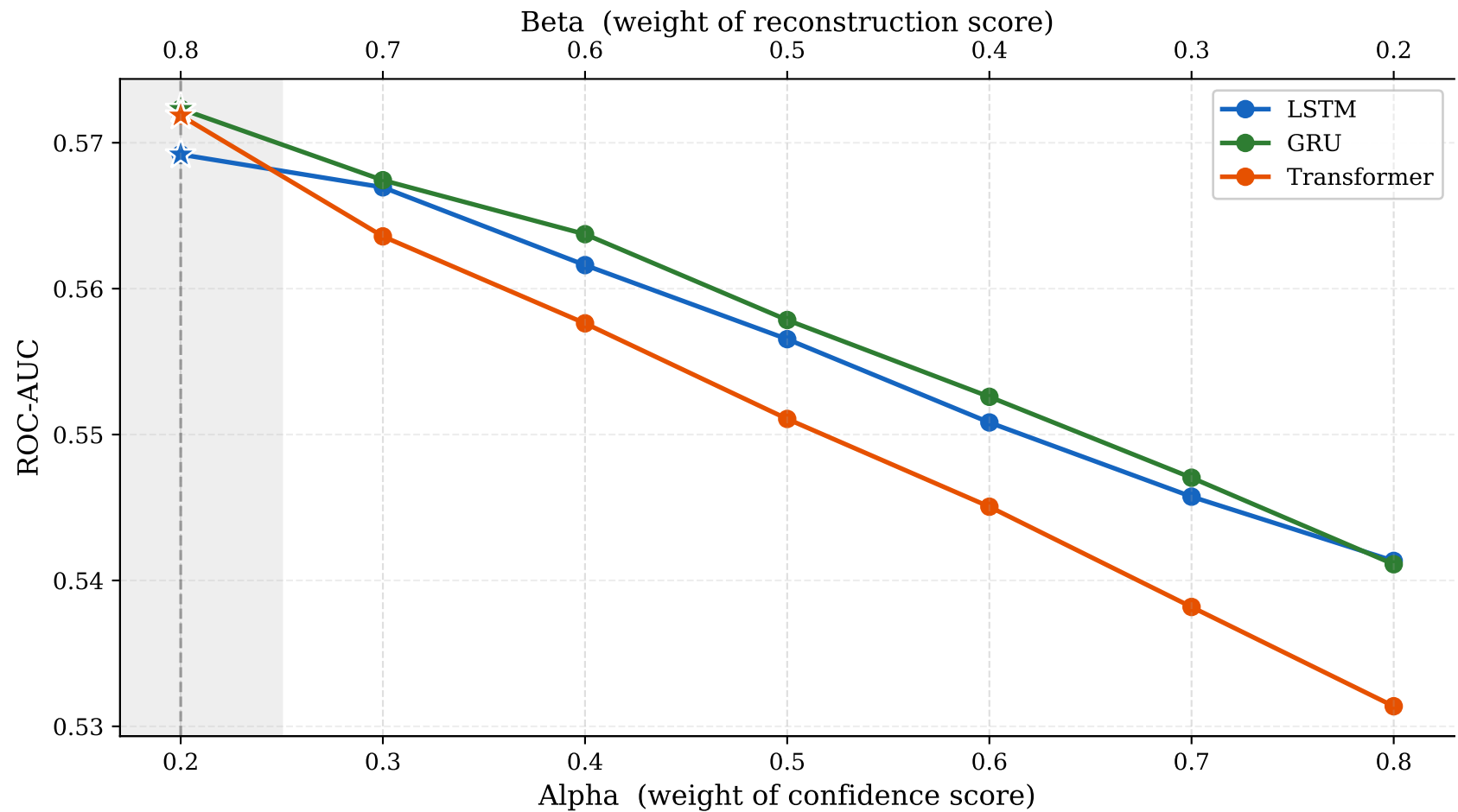
Figure 7 — Composite Scoring Weight Sensitivity Analysis
