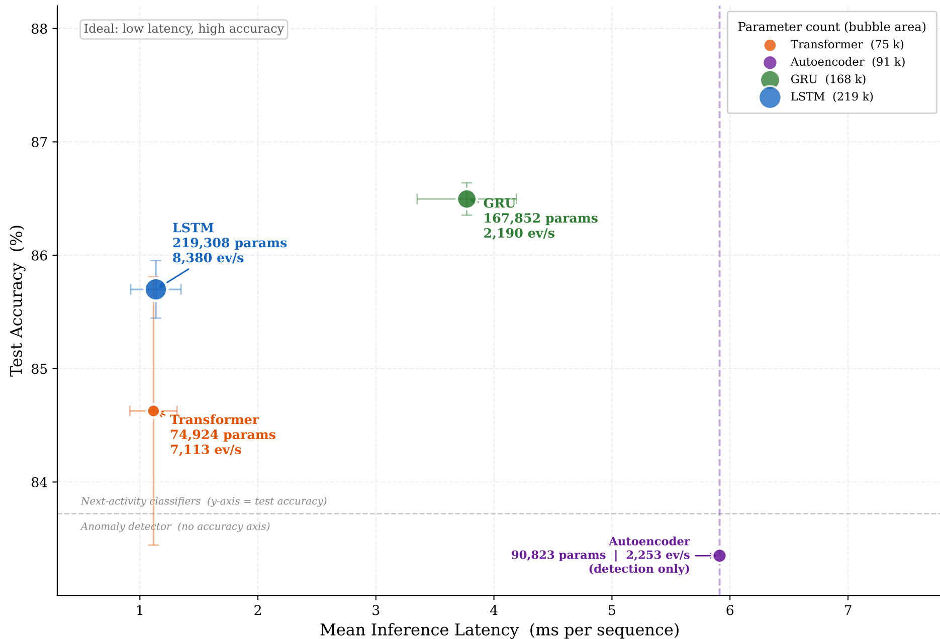
Figure 8 — Latency vs. Accuracy Deployment Tradeoff
