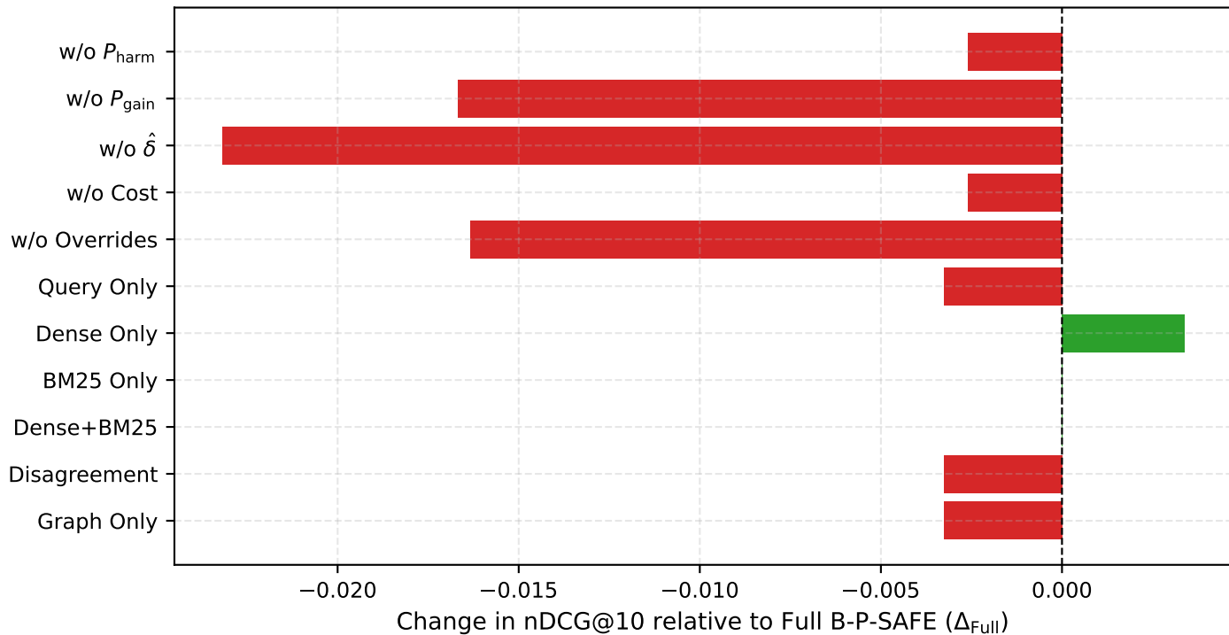
Router Component and Feature Ablation Effects
