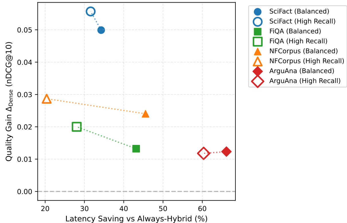
Quality-Latency Tradeoff (Seed 42)
