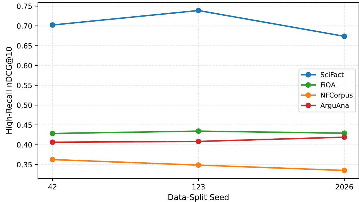
Multi-Seed Split Sensitivity (High Recall)
