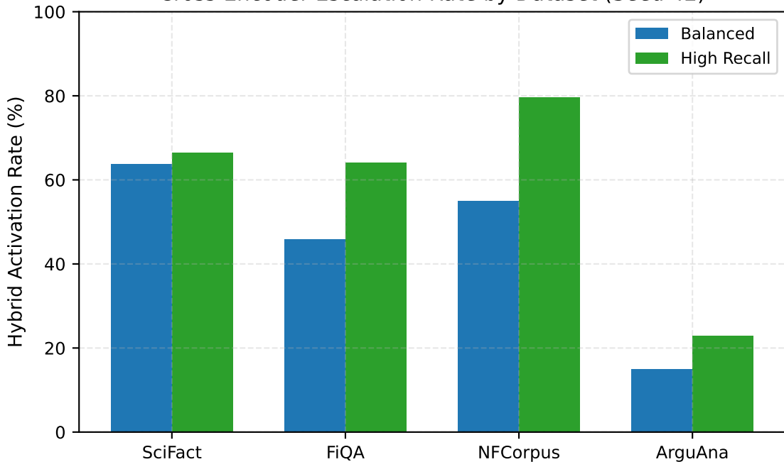
Cross-Encoder Escalation Rate by Dataset (Seed 42)
