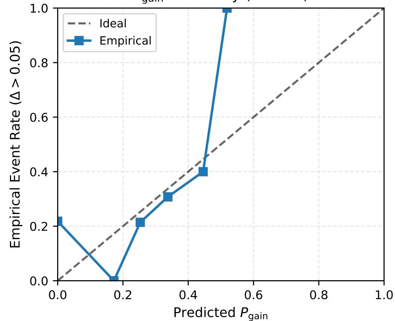
P_{\text{gain}} Reliability (SciFact)
