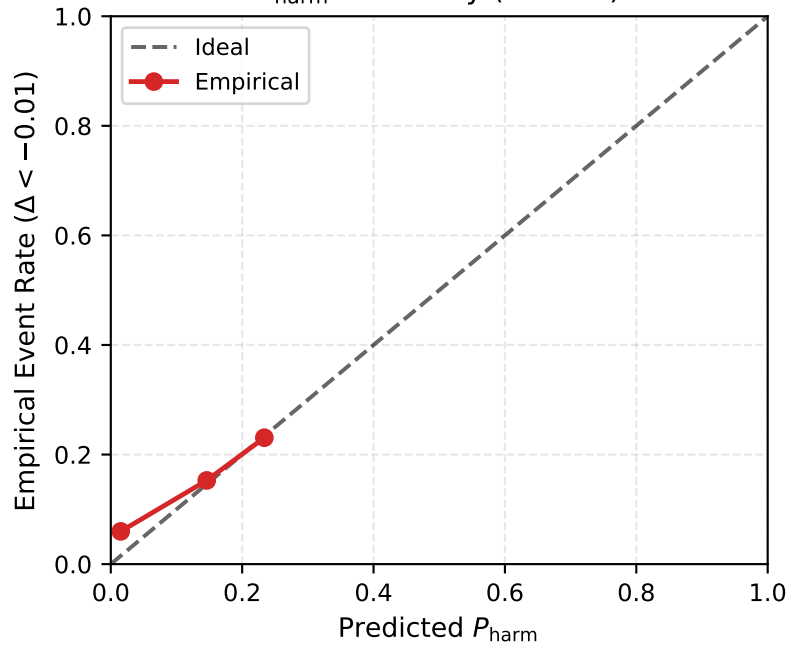
P_{\text{harm}} Reliability (SciFact)
