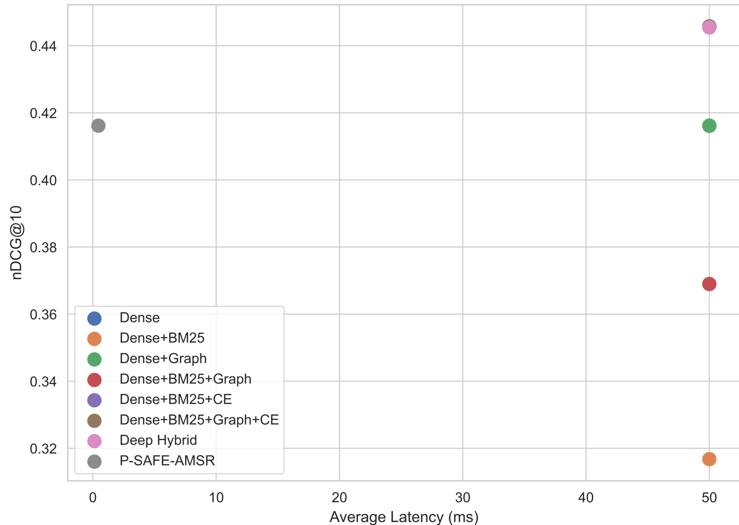
Utility / Pareto Frontier
