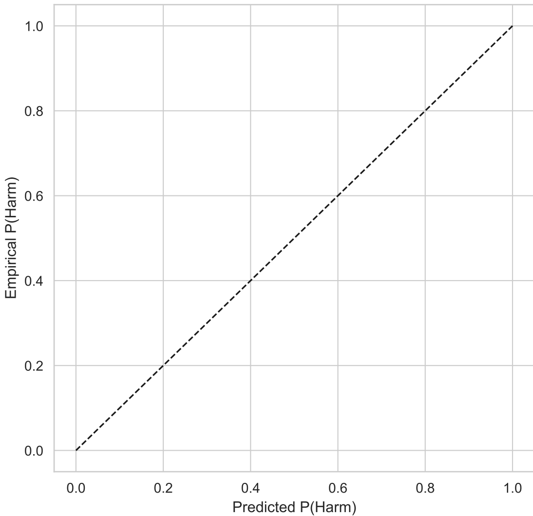
Calibration: P(Harm)
