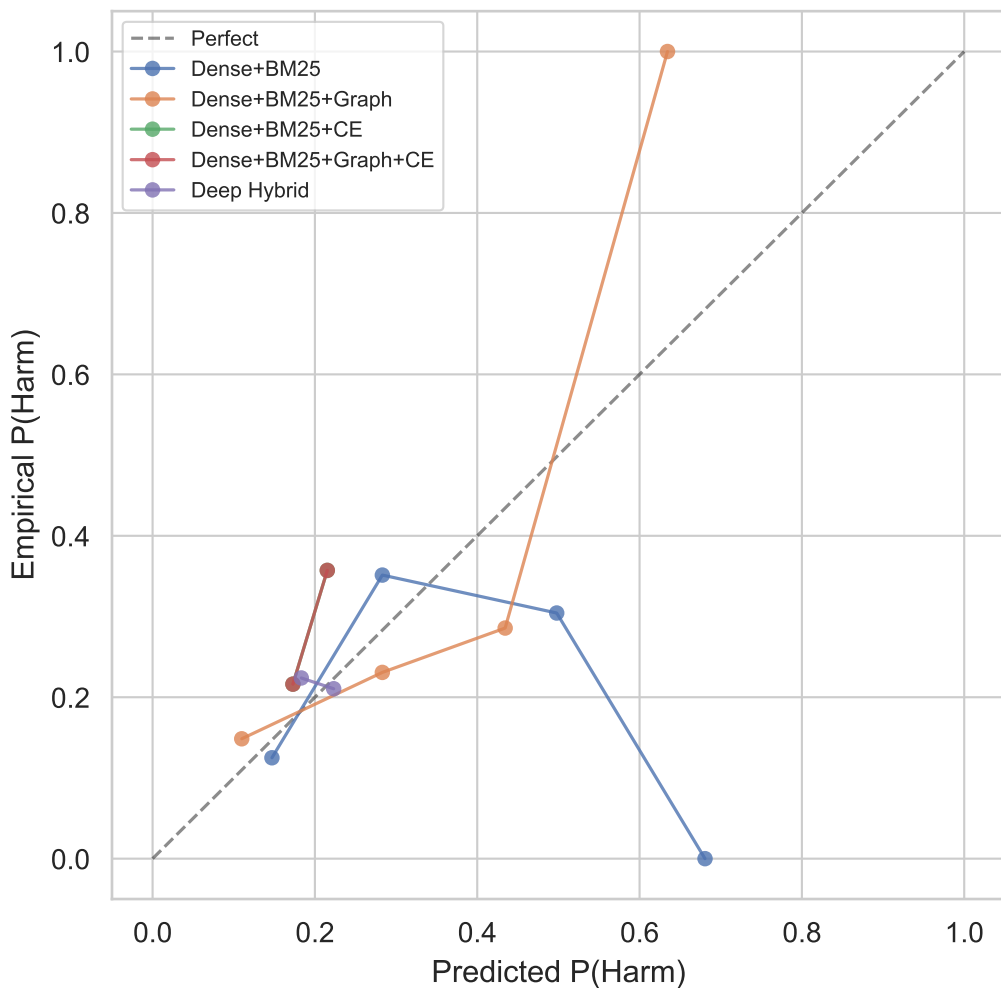
Calibration: Harm
