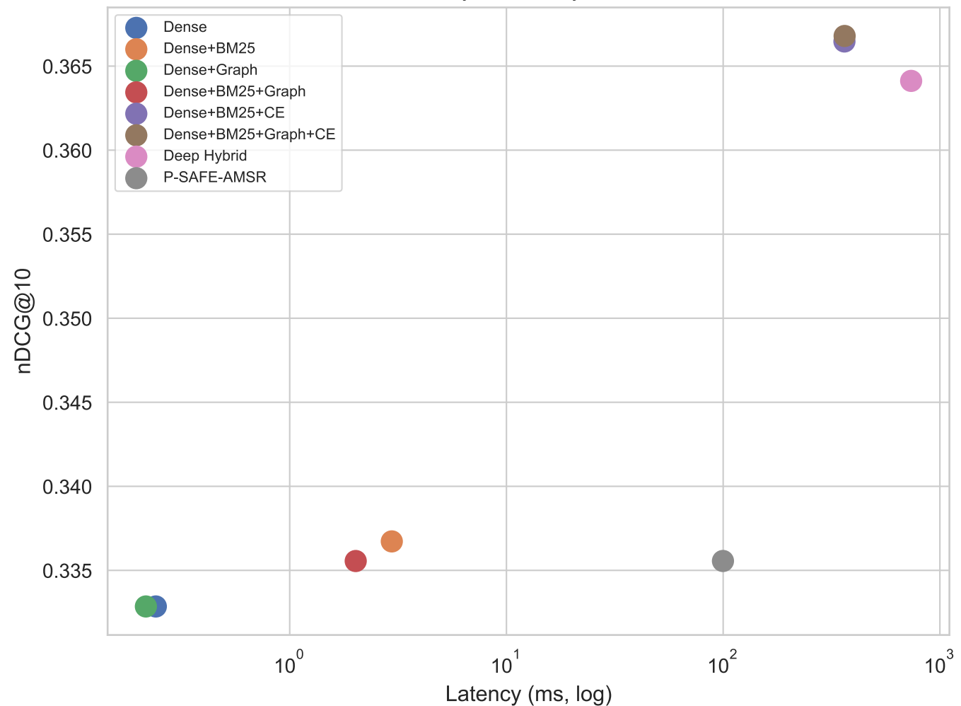
Quality vs Latency Pareto
