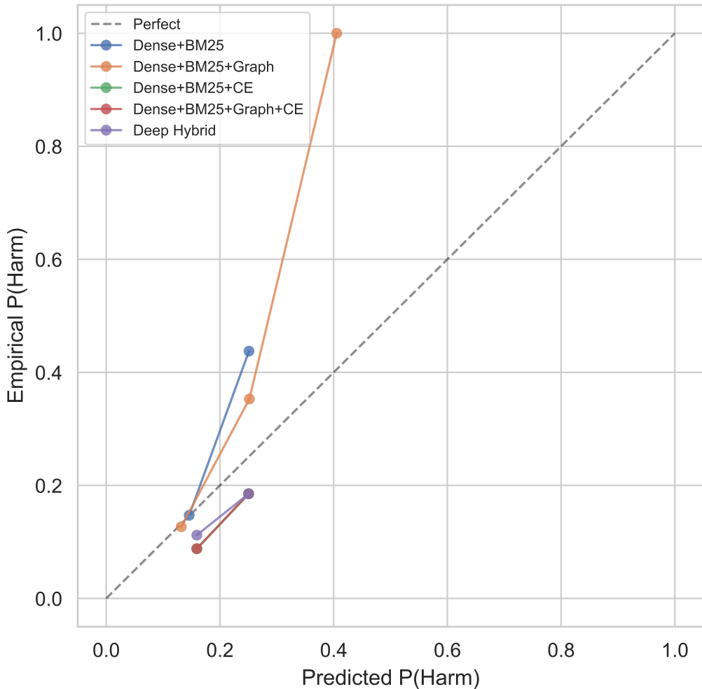
Calibration: Harm
