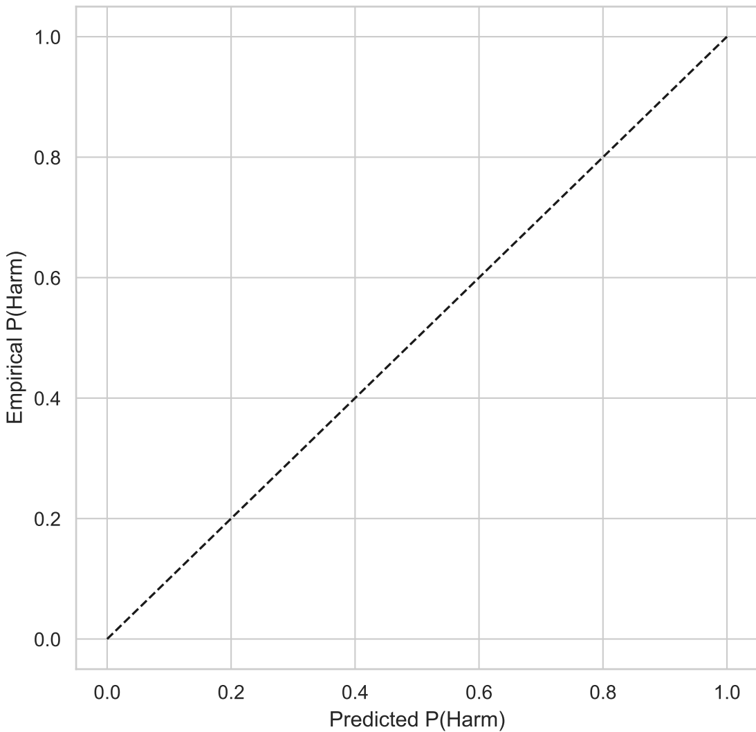
Calibration: P(Harm)
