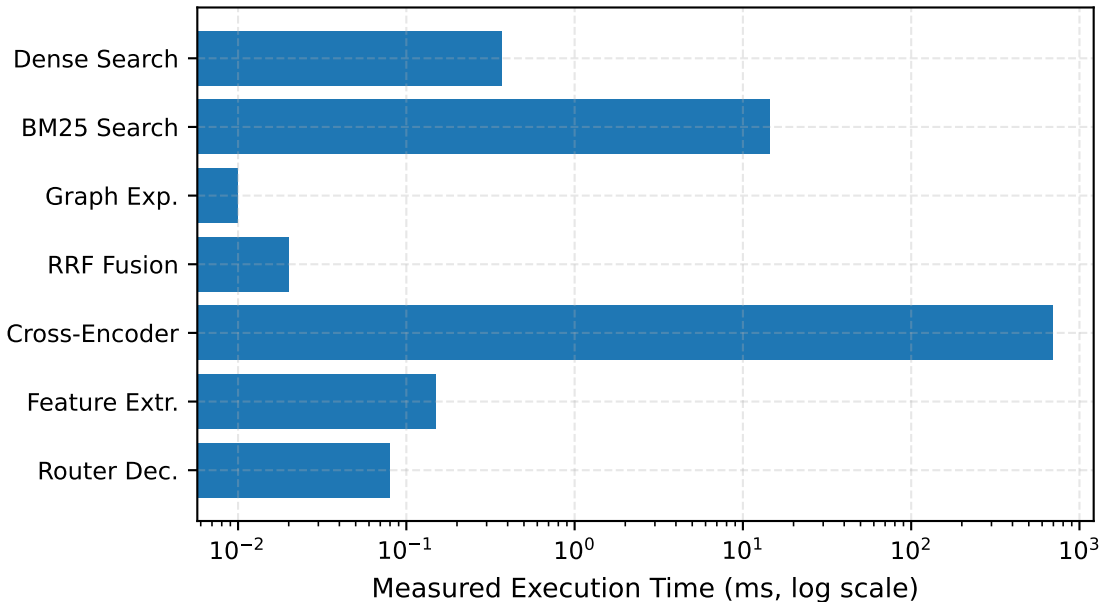
End-to-End Latency Breakdown (SciFact High Recall)
