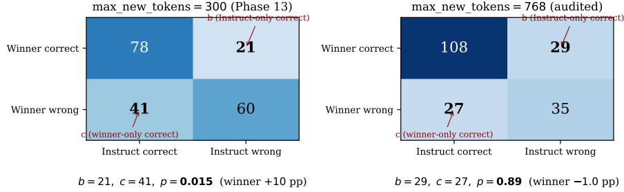
Figure 1: Figure 1: Paired McNemar contingency before and after the truncation audit. The +10 pp claim under max_new=300 (left, b = 21, c = 41, p = 0.0151 ) flips to -1.0 pp under max_new=768 (right, b = 29, c = 27, p = 0.8939 ). b and c are the discordant cells McNemar’s test sums over; the diagonal is the concordant agreement.
