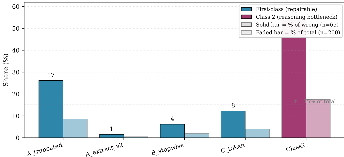
Figure 2: T0v2 channel distribution on the audited winner (200 GSM8K dev items).
