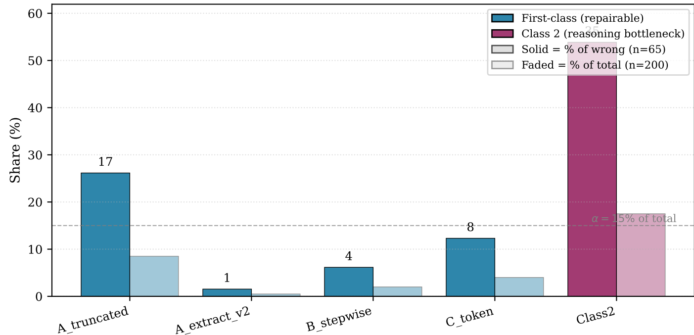
Figure 2: T0v2 channel distribution on the audited winner (200 GSM8K dev items).
