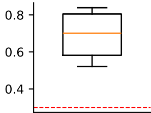
silhouette test
