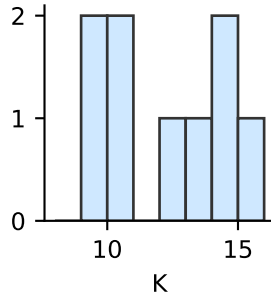
selected K
