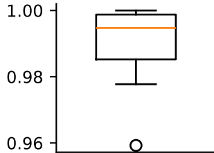
circular AUROC
