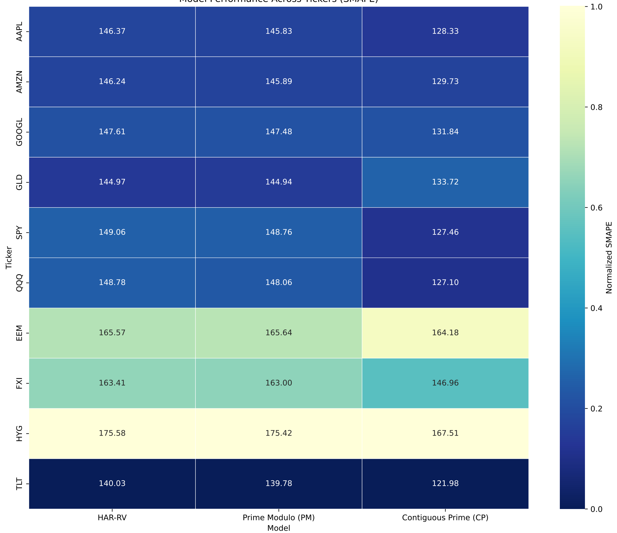
Model Performance Across Tickers (SMAPE)
