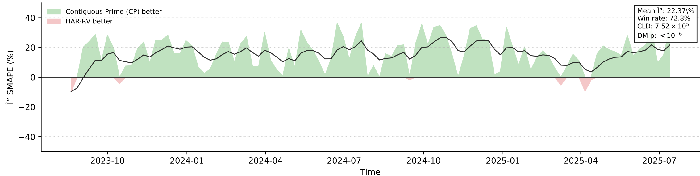
Error Advantage vs HAR-RV " Contiguous Prime (CP)
