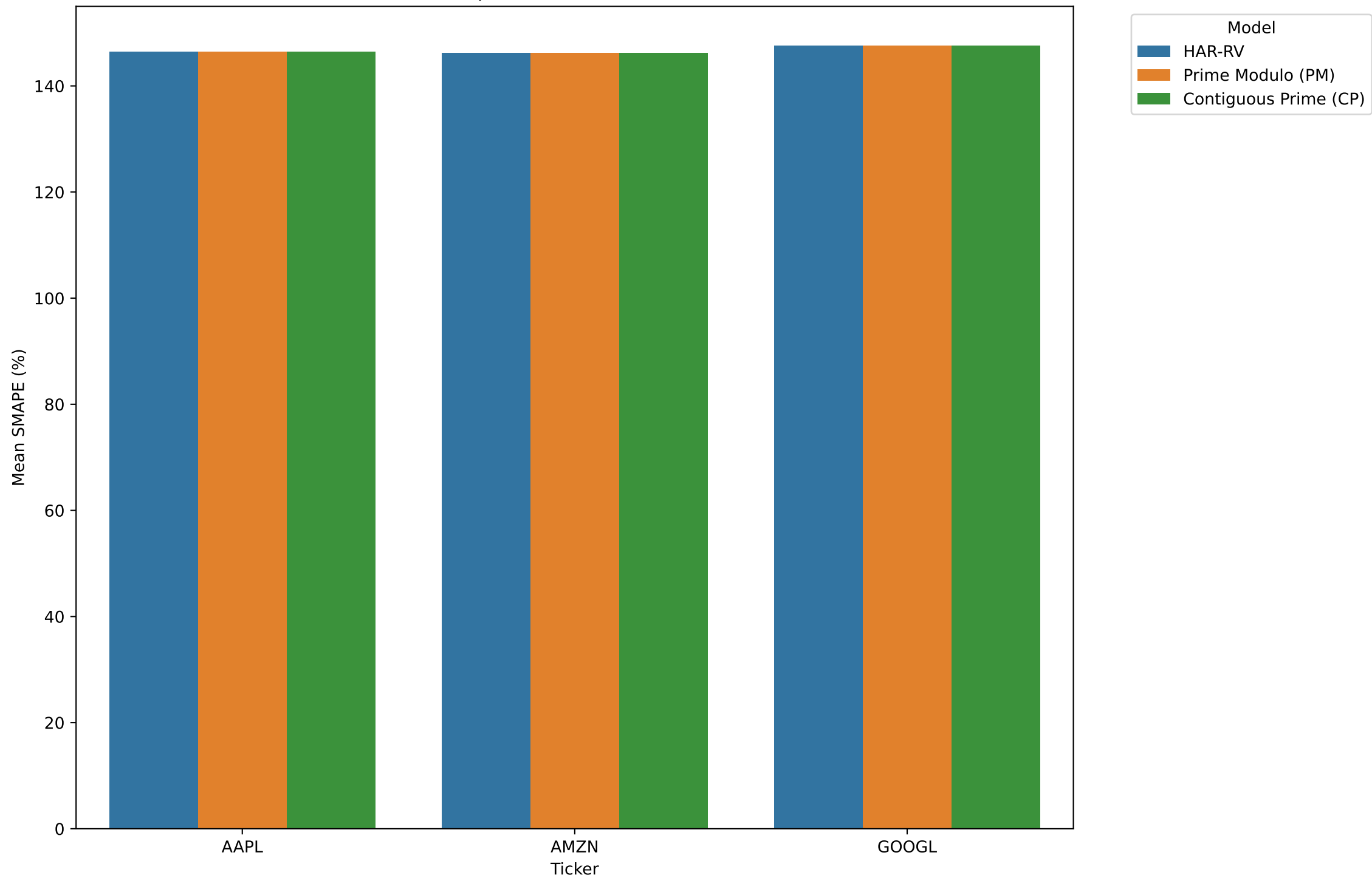
Model Comparison Across Tickers (SMAPE)
