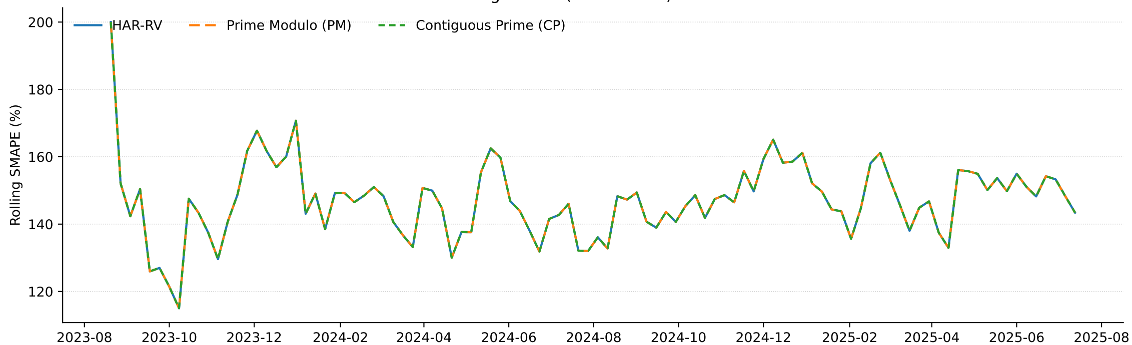
Rolling SMAPE (window=78) — AMZN
