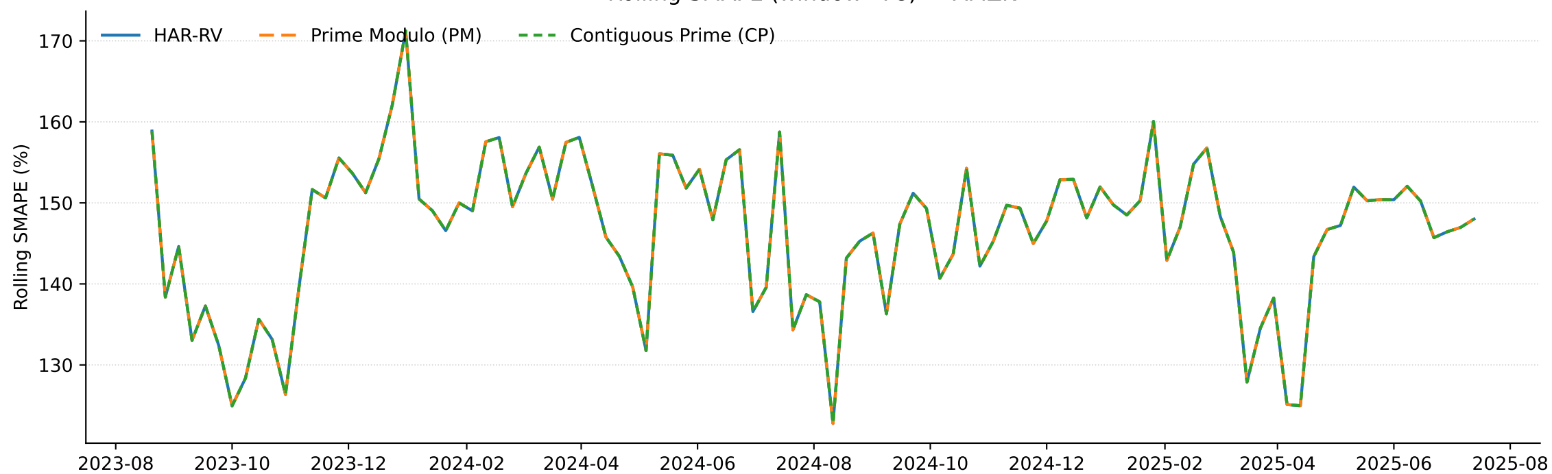
Rolling SMAPE (window=78) — GOOGL
