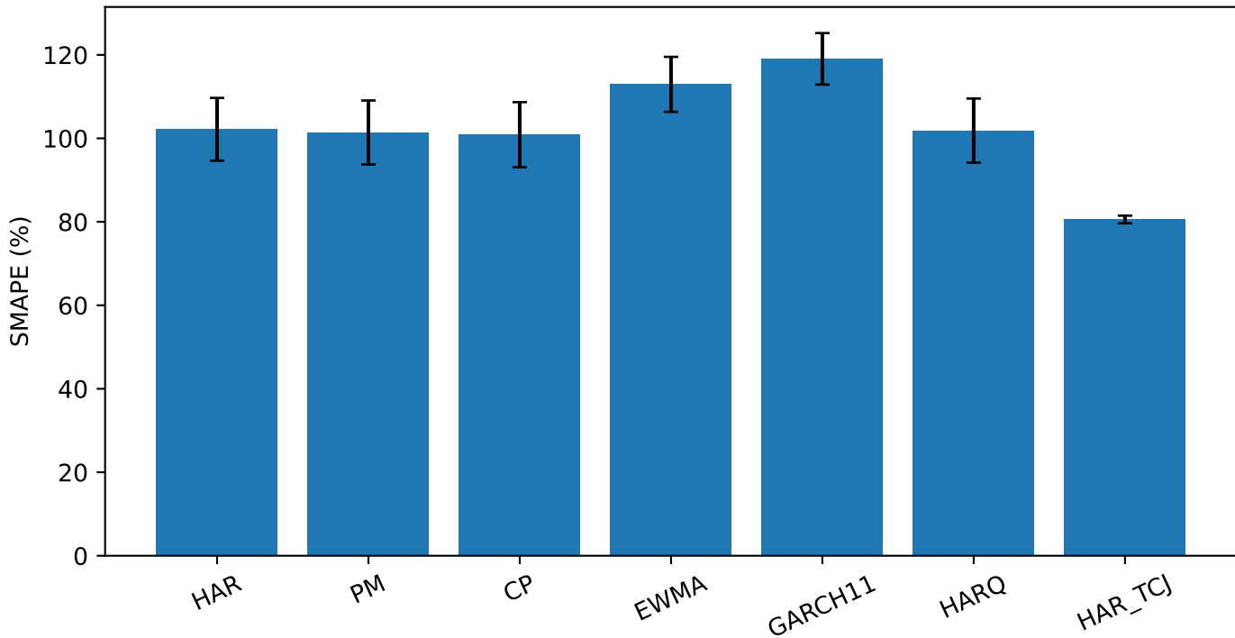
External Baseline Comparison
