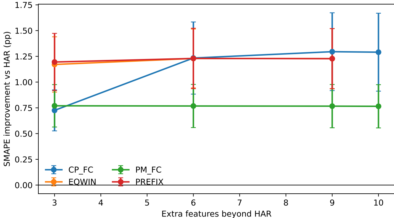
Feature Count Curve
