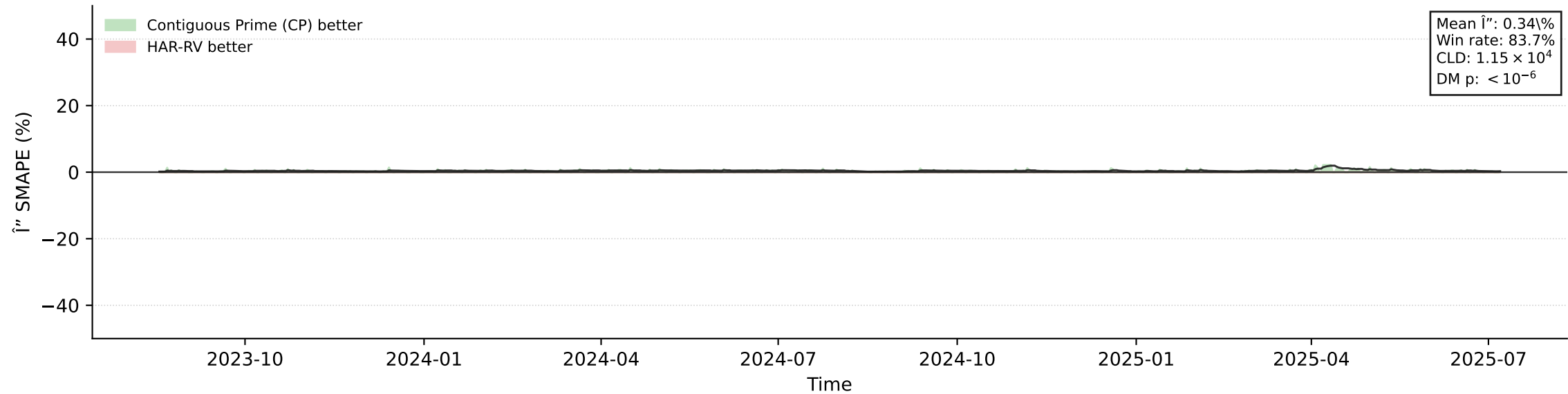
Error Advantage vs HAR-RV \hat{I}'' Contiguous Prime (CP)
