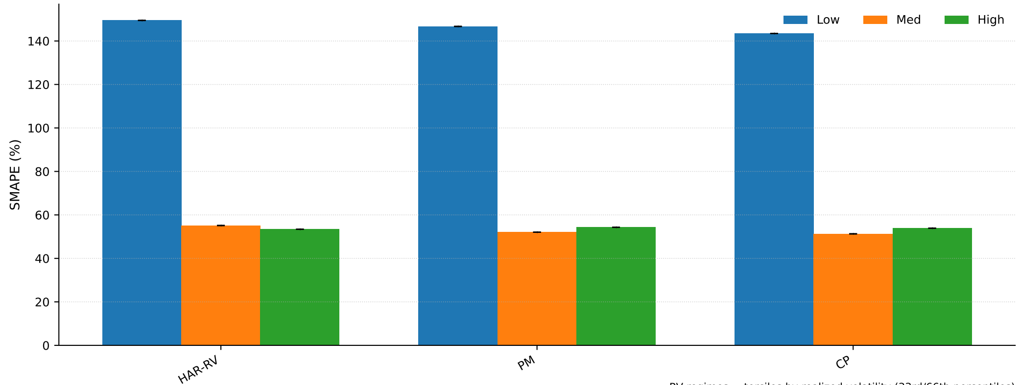
SMAPE% by RV Regime (Intraday)
