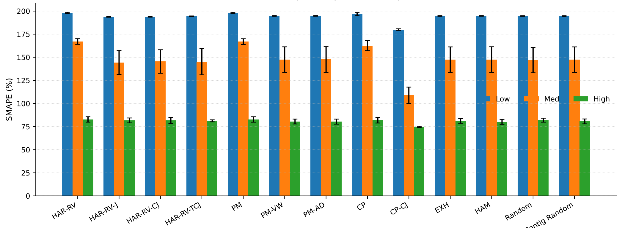
SMAPE% by RV Regime (Intraday)
