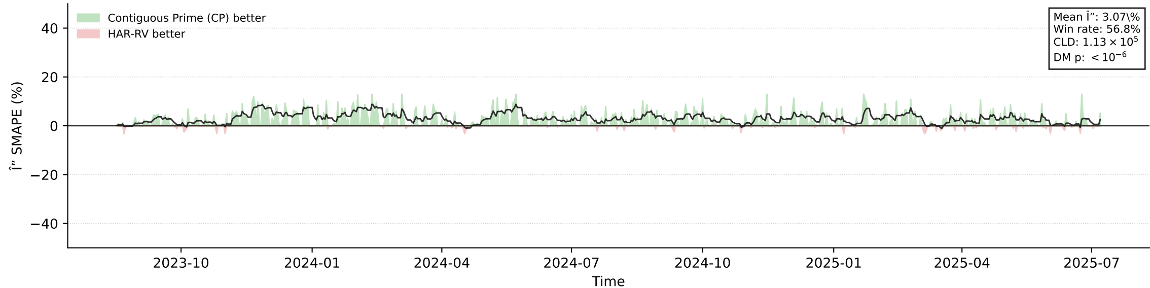
Error Advantage vs HAR-RV \hat{\epsilon} Contiguous Prime (CP)
