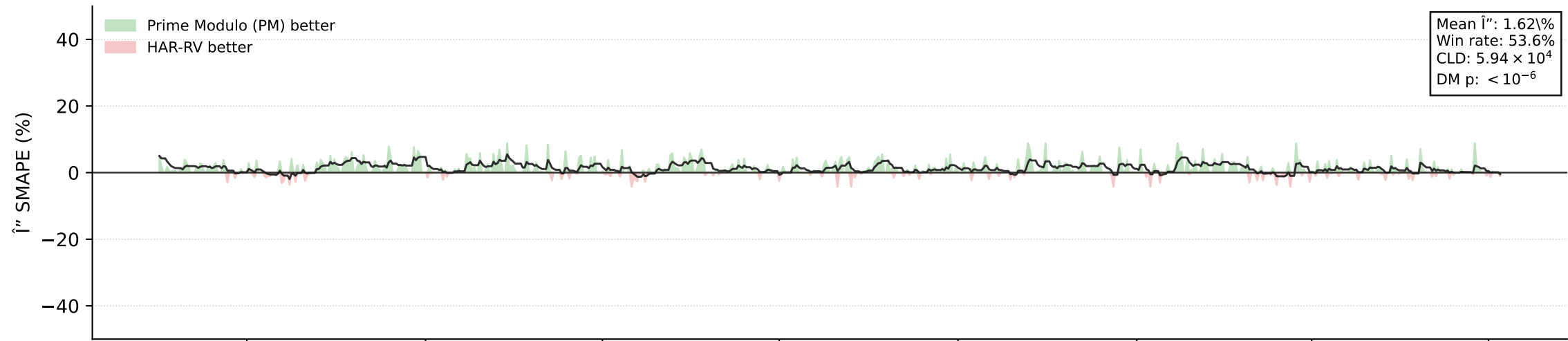
Error Advantage vs HAR-RV \hat{\epsilon} Prime Modulo (PM)
