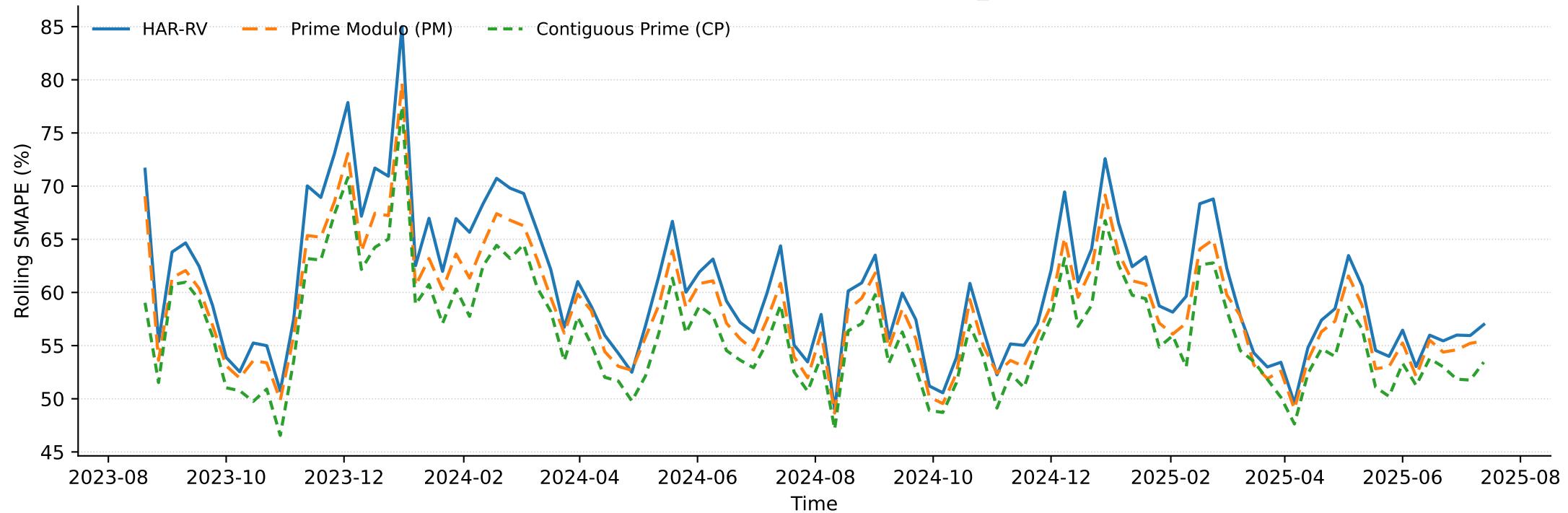
Rolling SMAPE (window=78) — ALL_MEAN
