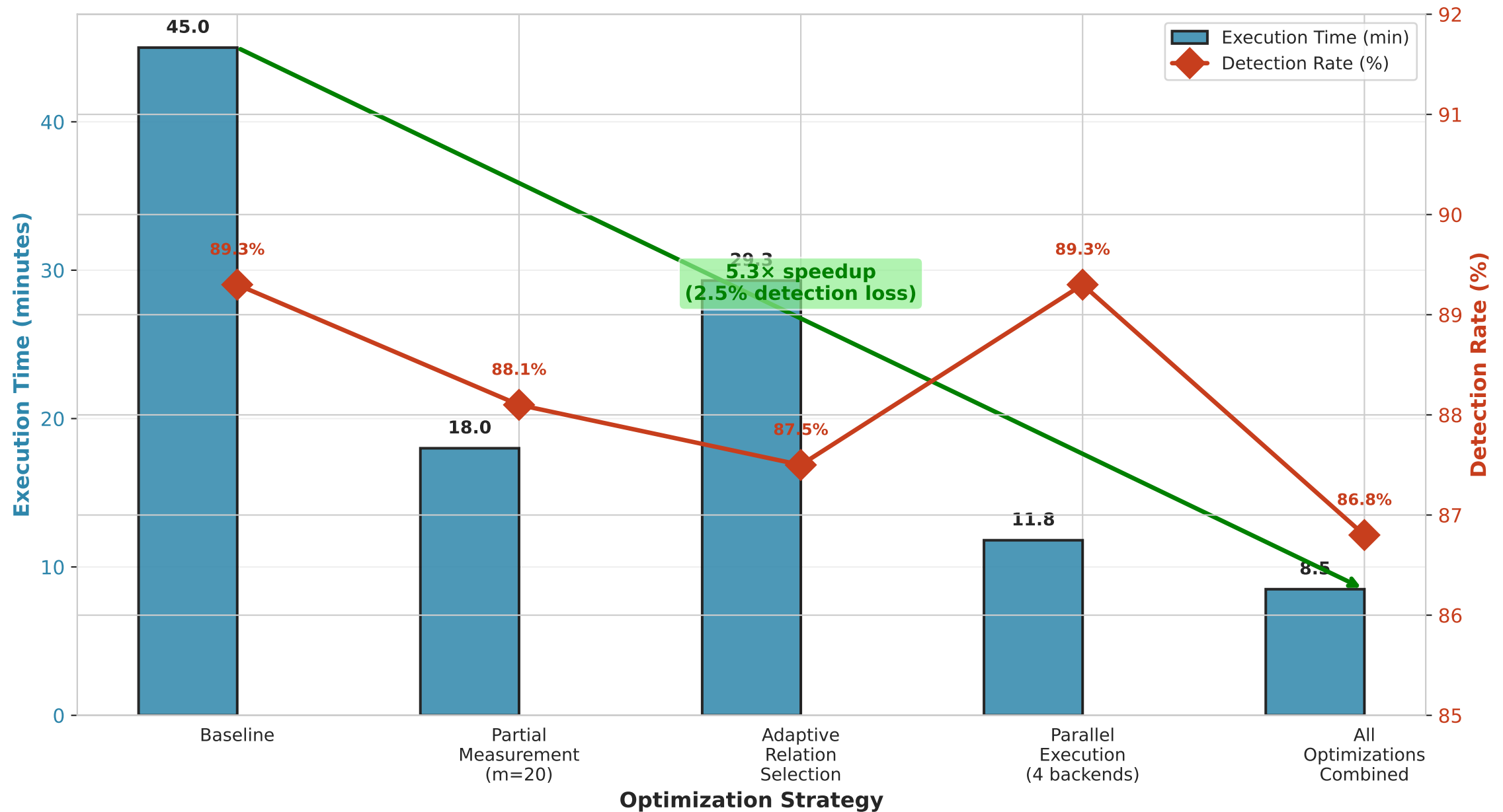
Optimization Strategies for 50-Qubit Circuits (Depth 100)
