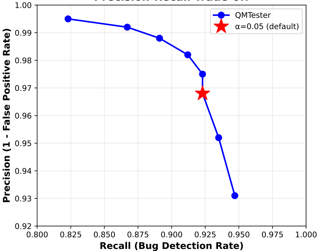
Precision-Recall Trade-off
