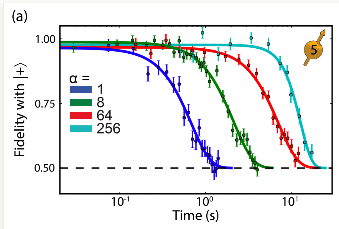
A measured version of the same decay: the fidelity of one spin with |+\rangle , which falls to the 0.5 floor as the Bloch radius shrinks to zero. The bare curve \alpha = 1 decays first, like the T_2^* above; the longer ones are the same spin under the dynamical decoupling of the next slides. The time axis is logarithmic, and its scale is that spin's own.
