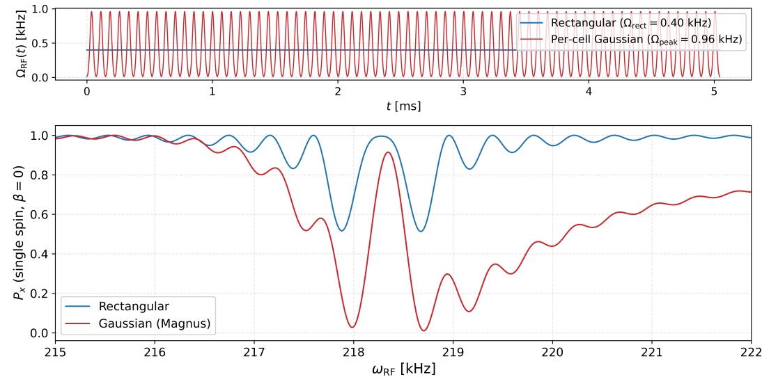
DDrf spectroscopy: rectangular vs per-cell Gaussian (equal area), N = 136 , \tau = 8 \cdot 2\pi/\omega_0 , \Omega_{\text{rect}} = 0.40 kHz
