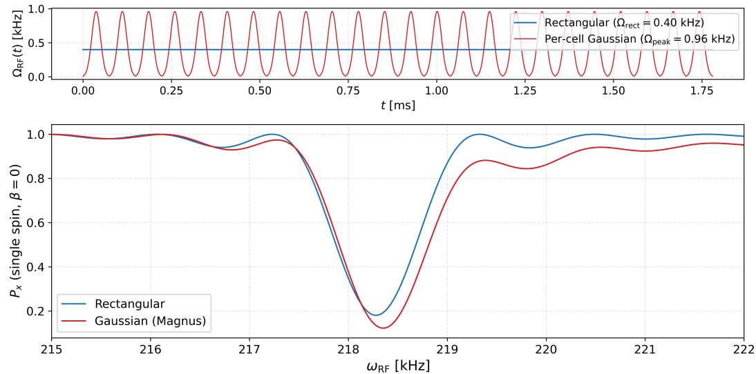
DDrf spectroscopy: rectangular vs per-cell Gaussian (equal area), N = 48 , \tau = 8 \cdot 2\pi/\omega_0 , \Omega_{\text{rect}} = 0.40 kHz
