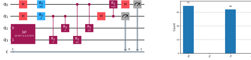
Figure 3: |\psi\rangle = \frac{1}{\sqrt{2}}(|00\rangle + |11\rangle) (a) Hamming Weight Measurement Circuit. (b) Histogram of Hamming Weight Measurement Results.
