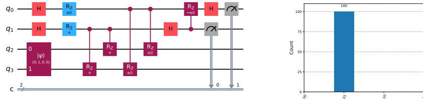
Figure 2: |\psi\rangle = |01\rangle (a) Hamming Weight Measurement Circuit. (b) Histogram of Hamming Weight Measurement Results.
