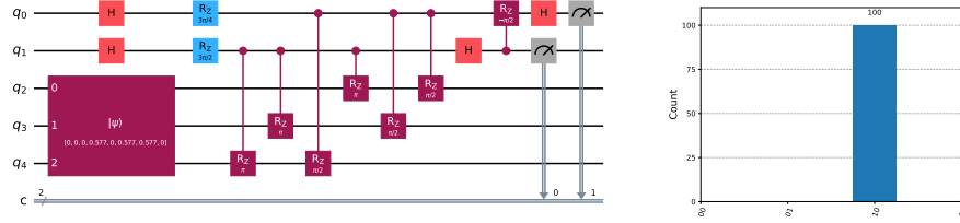
Figure 4: |\psi\rangle = \frac{1}{\sqrt{3}}(|011\rangle + |101\rangle + |110\rangle) (a) Hamming Weight Measurement Circuit. (b) Histogram of Hamming Weight Measurement Results.
