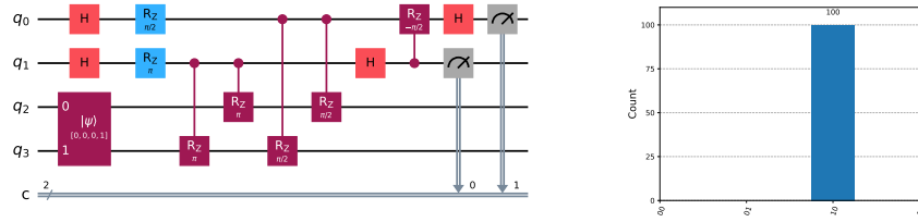
Figure 1: |\psi\rangle = |11\rangle (a) Hamming Weight Measurement Circuit. (b) Histogram of Hamming Weight Measurement Results.
