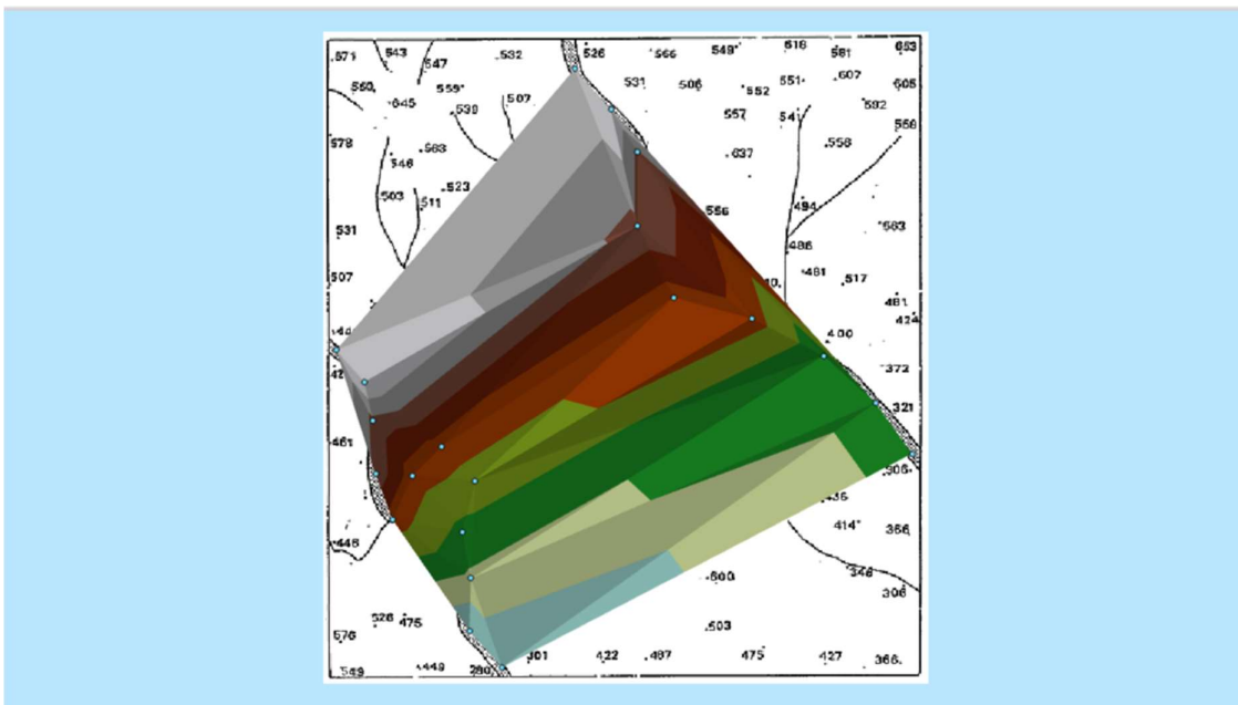
Constrained TIN using 21 river points
