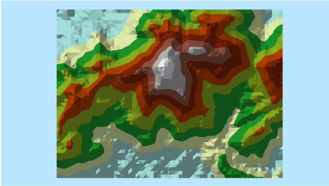
TIN with sampling interval of 141 meters
