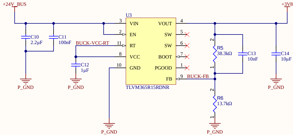
24V to 3.8V Buck Converter
