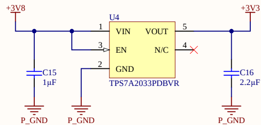
3.8V to 3.3V LDO Step Down
