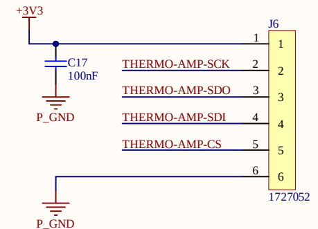
STM32 To Slip Ring Output (Power + Signals)
