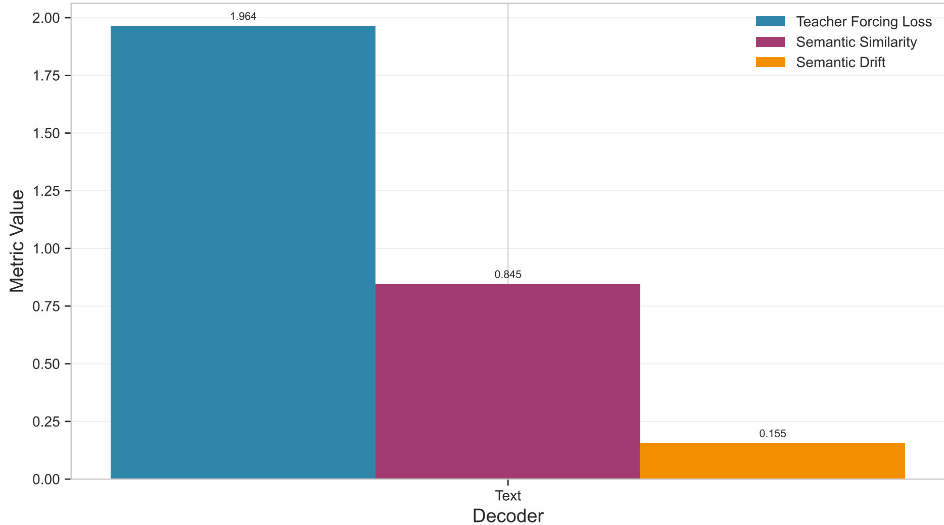
Final Training Metrics by Decoder
