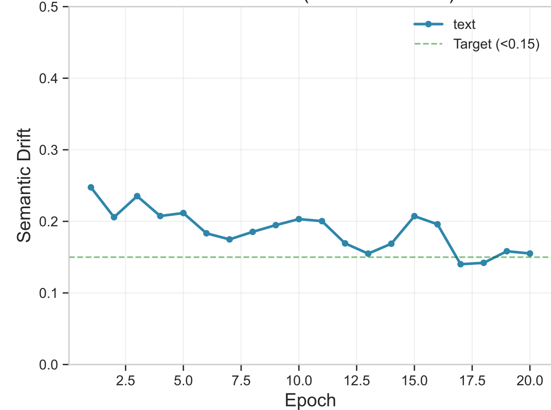
Semantic Drift (Lower is Better)
