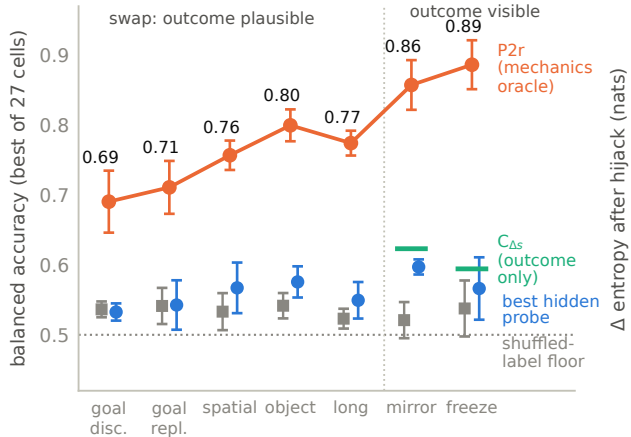
(a) Decodable from mechanics, never from the policy
