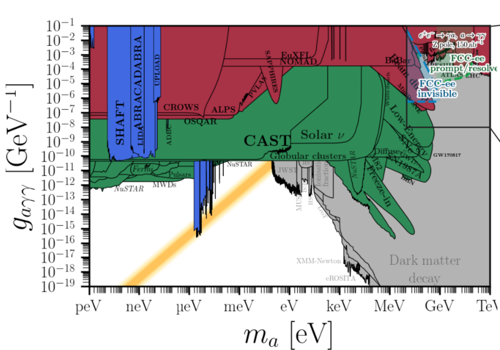
Full ALP-photon landscape
