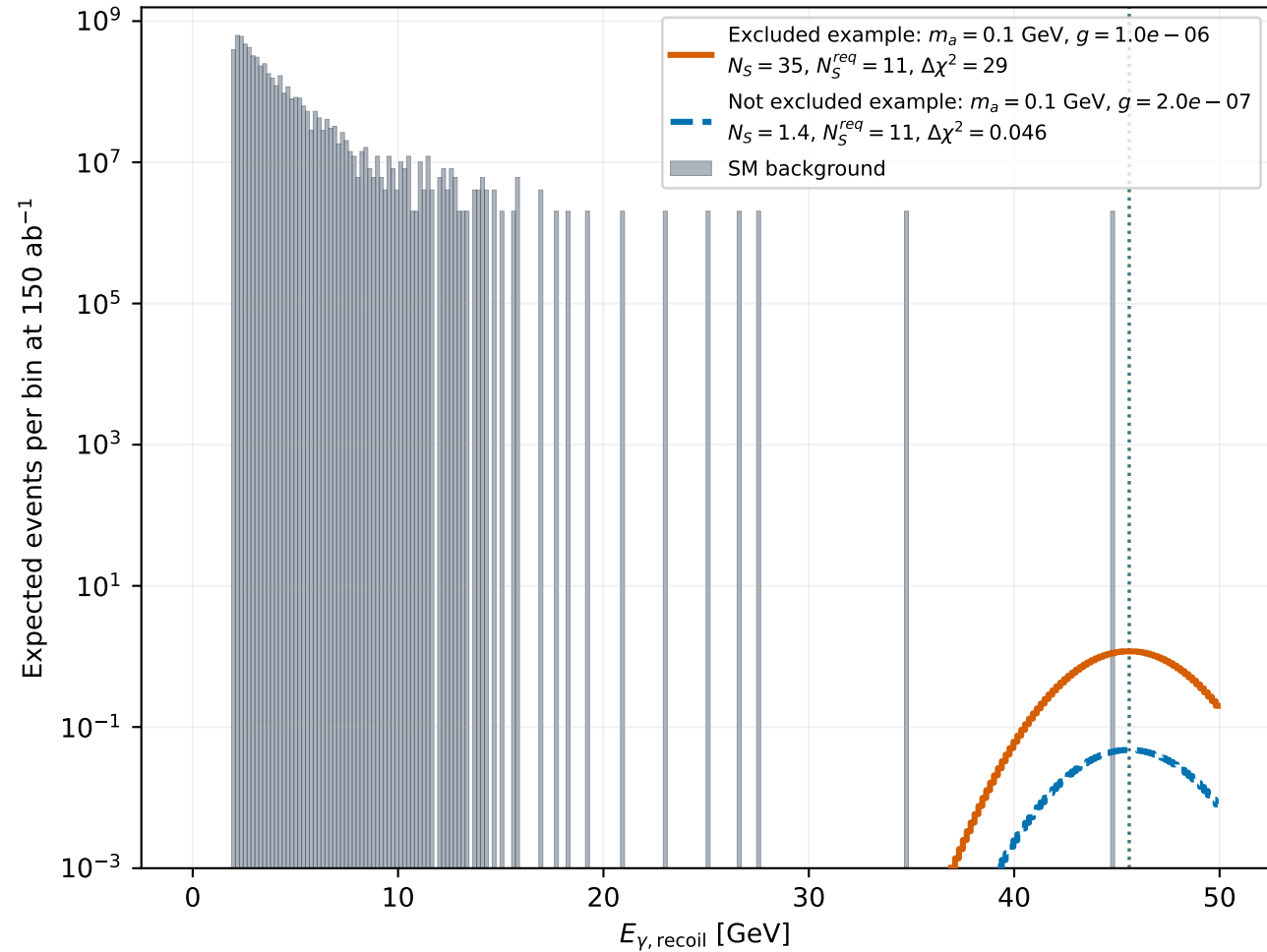
Invisible channel: e^+e^- \rightarrow \gamma\nu\bar{\nu} background
