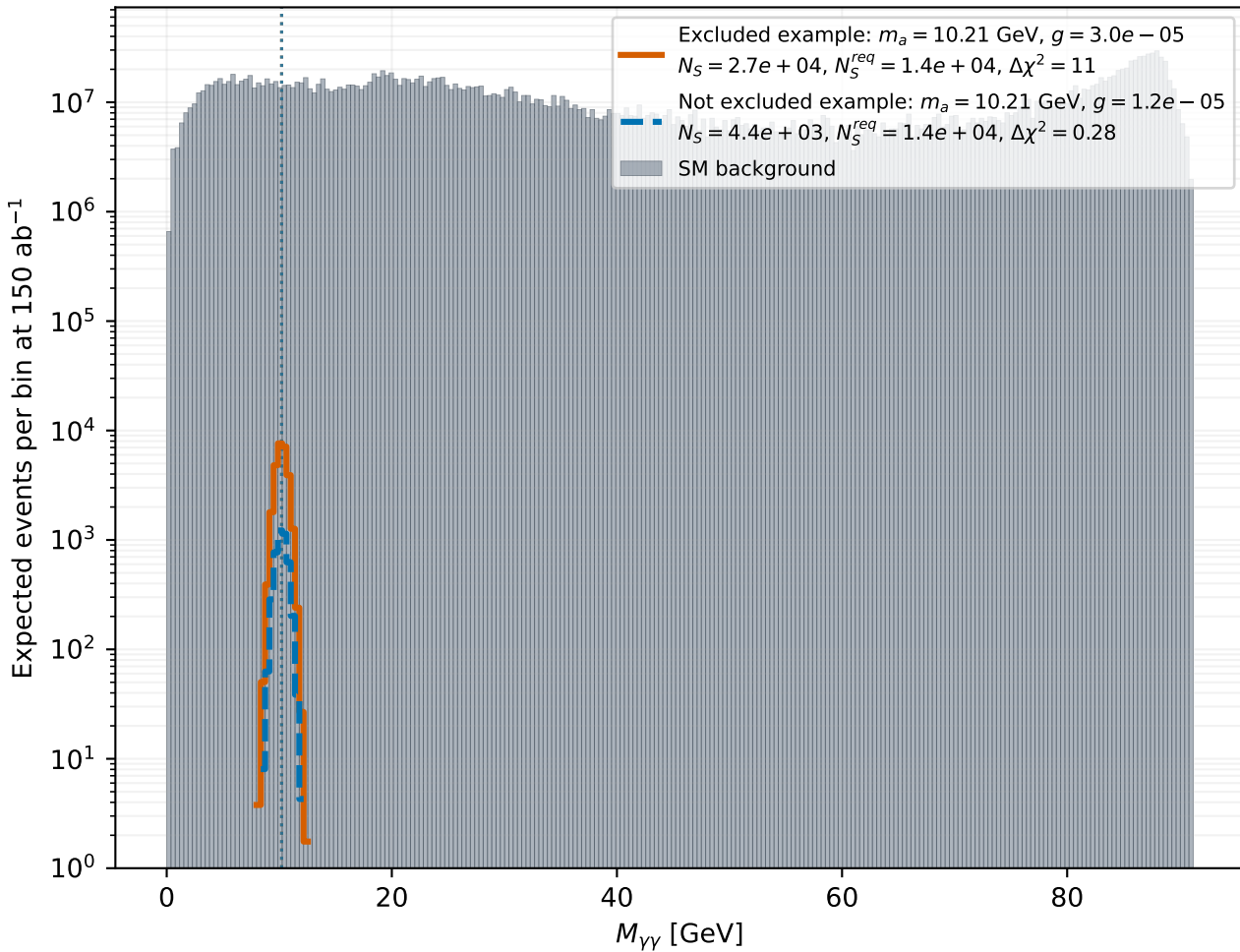
Prompt-resolved channel: e^+e^- \rightarrow \gamma\gamma\gamma background
