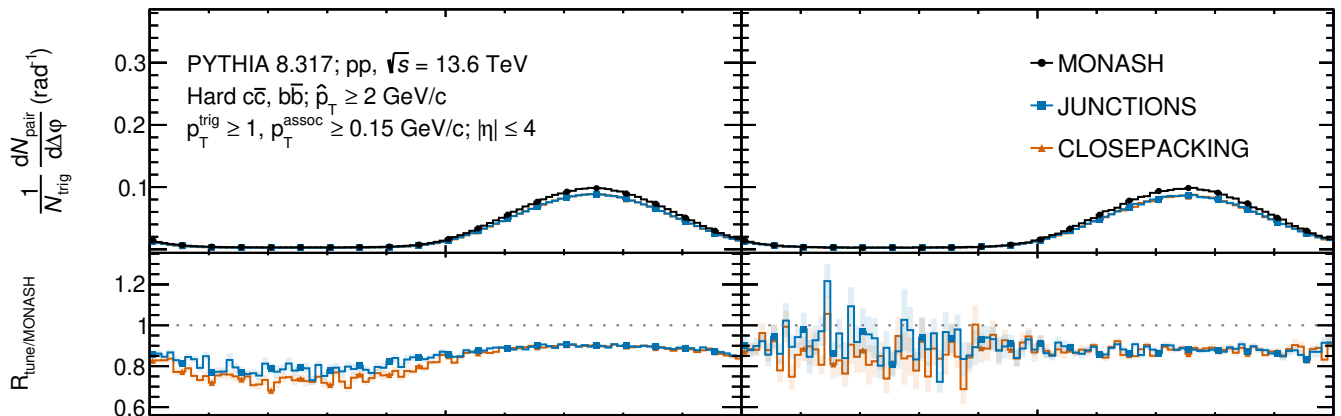
(a) D^0 trigger \rightarrow \bar{D}^0 , OS
