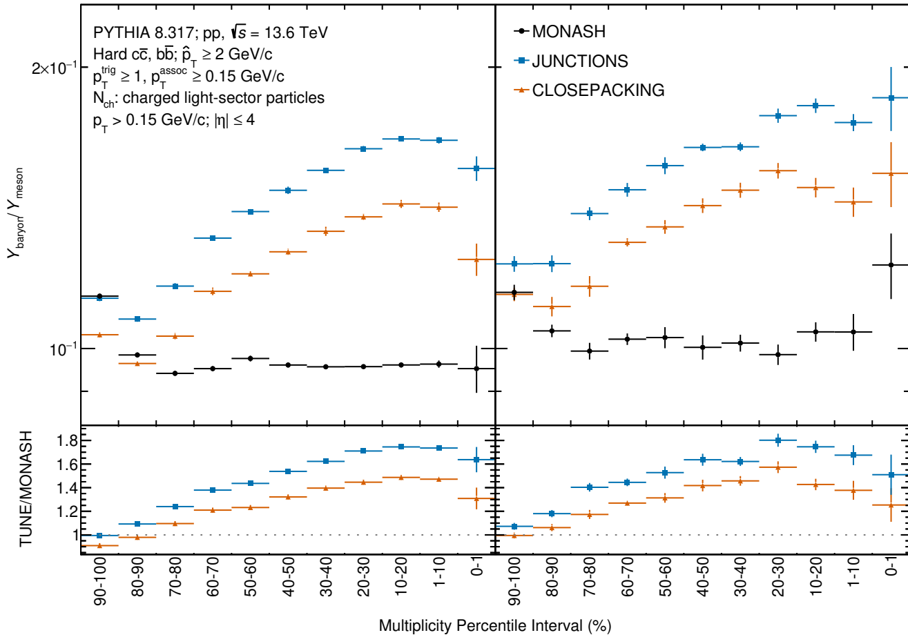
(a) D^0 trigger: \bar{\Lambda}_c^- / \bar{D}^0
