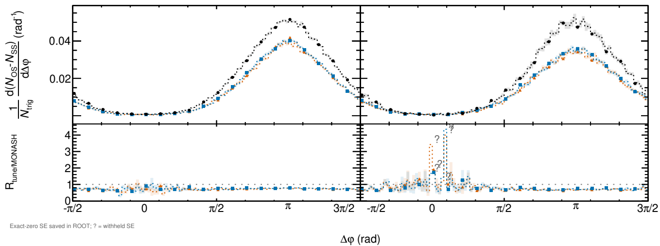
B^+ trigger, OS - SS
