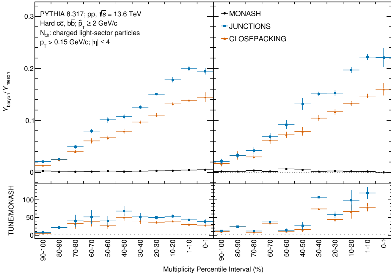
(a) B^+ trigger: \Xi_b^0 / B^-
