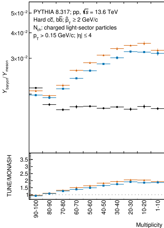
(a) D^0 trigger: \bar{\Xi}_c^- / \bar{D}^0
